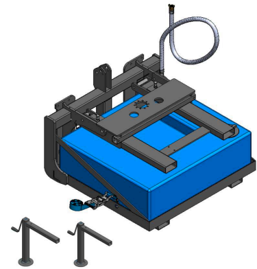
Flexi Adapter XII with mounting bracket and attachments
